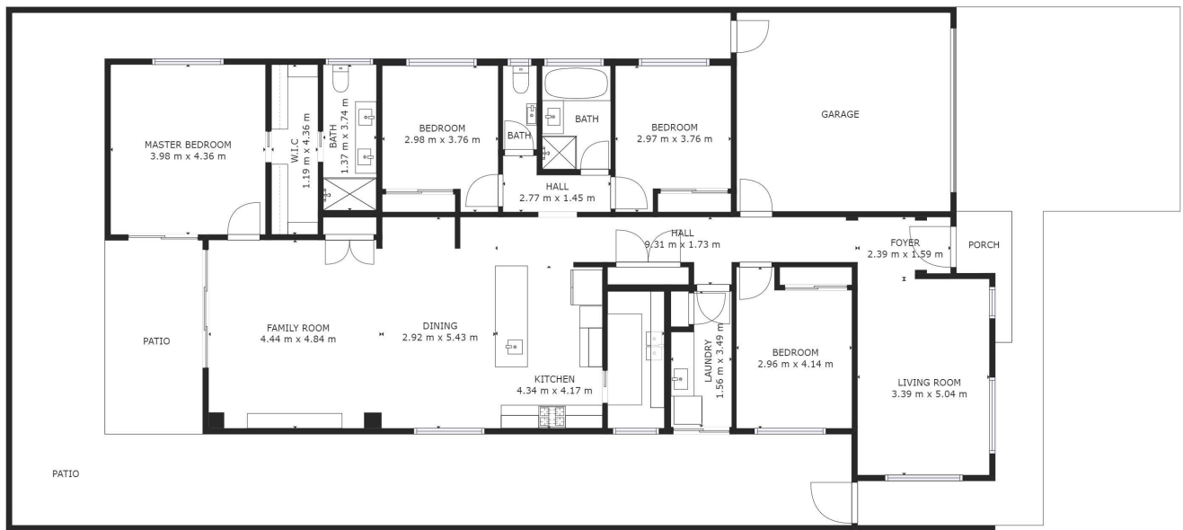
FLOOR 1
